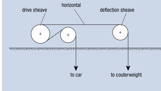
Fig. 36: The laterally positioned machine
