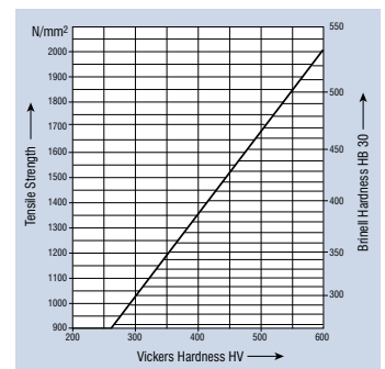
Fig. 7: Tensile strength, Brinell / Vickers hardness
