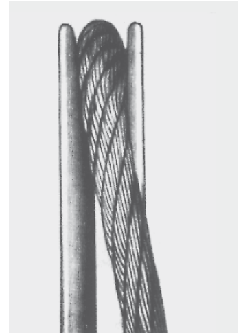
Fig. 37: Lateral deflection when running over a sheave (exaggerated for illustrative purposes)
